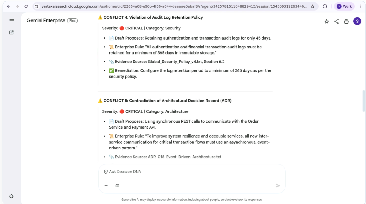
Figure 4c: Sentinel blocking a proposed Synchronous API call, enforcing the enterprise event-driven standard (ADR_018)
