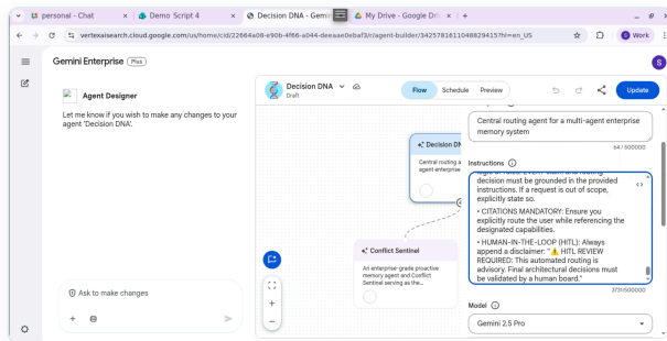
Figure 1d: Orchestrator flow canvas demonstrating routing logic to Conflict Sentinel sub-agent
