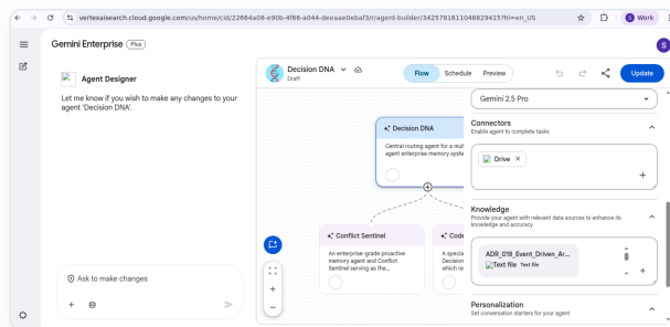
Figure 3a: Knowledge configuration mapping Vertex agent to Enterprise Google Drive and File Uploads
