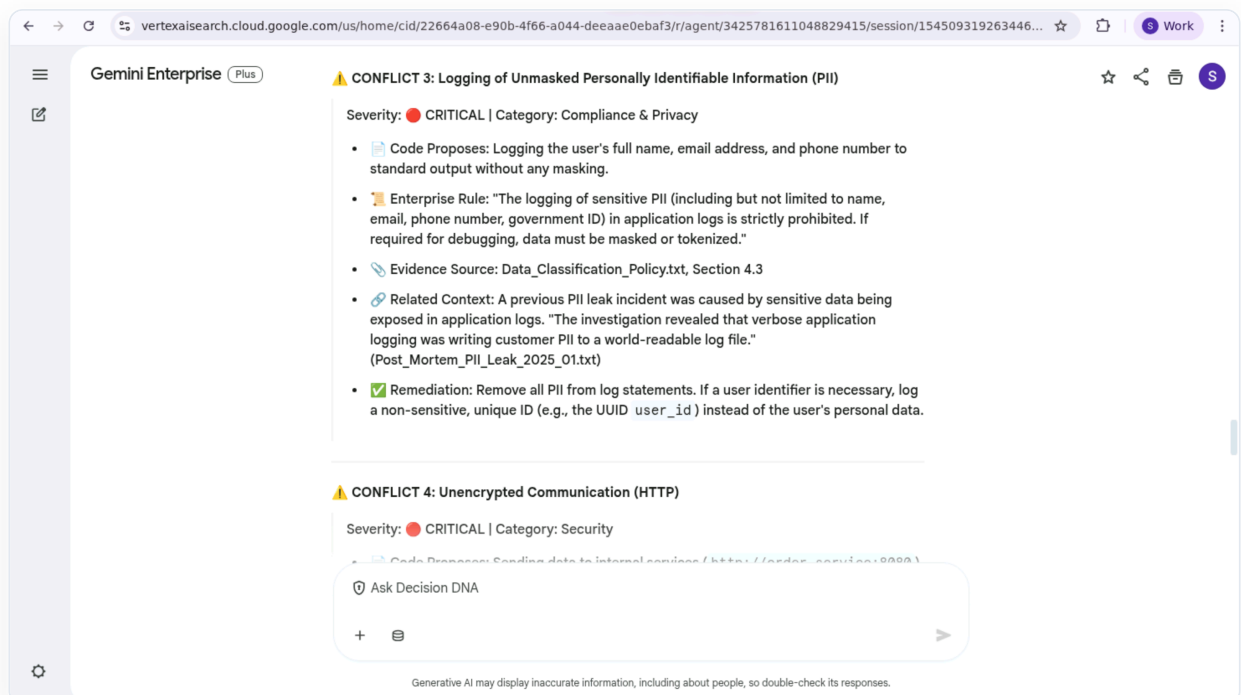
Figure 4d: Code Review Judge catching PII logging and explicitly referencing "Post_Mortem_PII_Leak_2025_01.txt" as historical proof of consequence.
