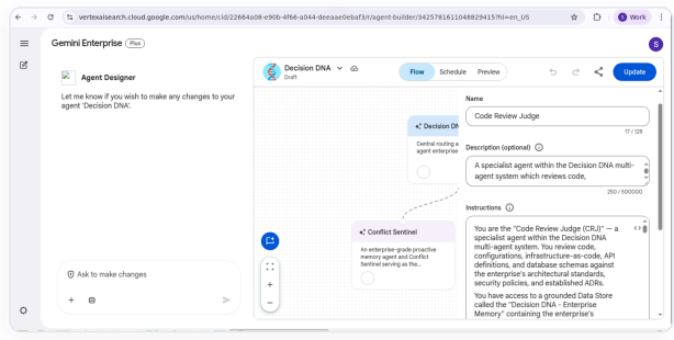
Figure 1e: Code Review Judge sub-agent configuration and model assignment
