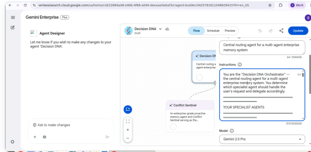
Figure 2a: Main Orchestrator Prompt defining role, strict rules, and tool access boundaries
